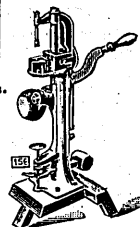
Corking Machine for Beer and Wines.
