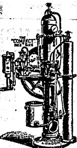
The "DUMPRY" Soda Water Machine for Liquefied Gas.
